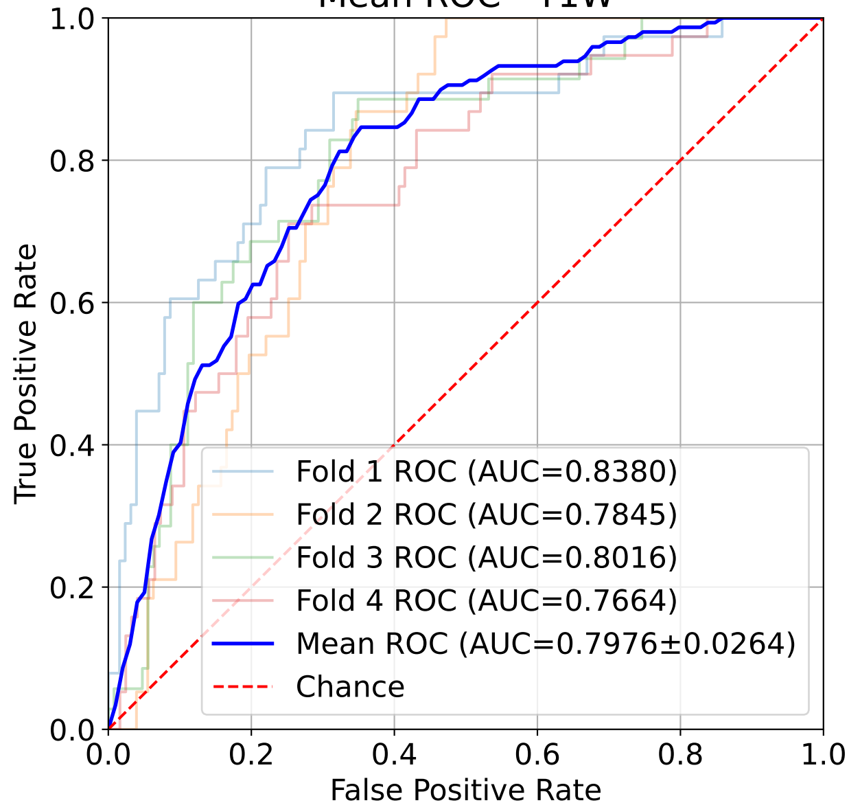
Mean ROC - T1W
